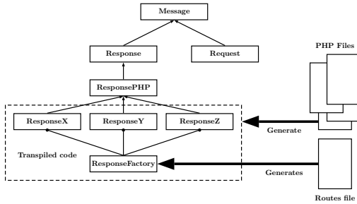
Fig. 2. PHP2Uni’s architecture and key classes.
