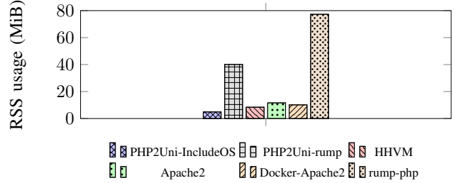
Fig. 3. Memory usage (RSS and as reported by docker stats) comparison across solutions.
